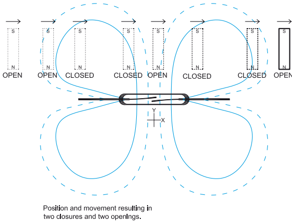
(Figure #30. The opening and closing points are shown for a vertically mounted magnet making an approach parallel to the Reed Switch. Here the Reed Switch will close and open two times.)
